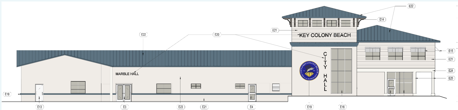
WEST ELEVATION
